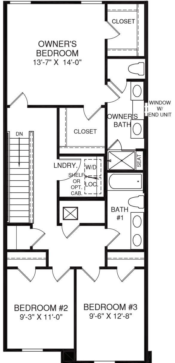
UPPER LEVEL
